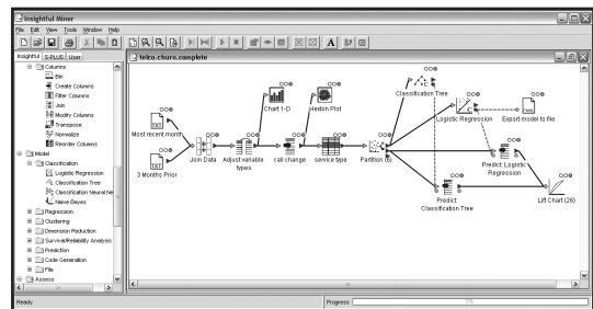
Figure 1. Easy to learn and easy to use, Insightful Miner enables statisticians and business analysts to create powerful, self-documenting applications.
